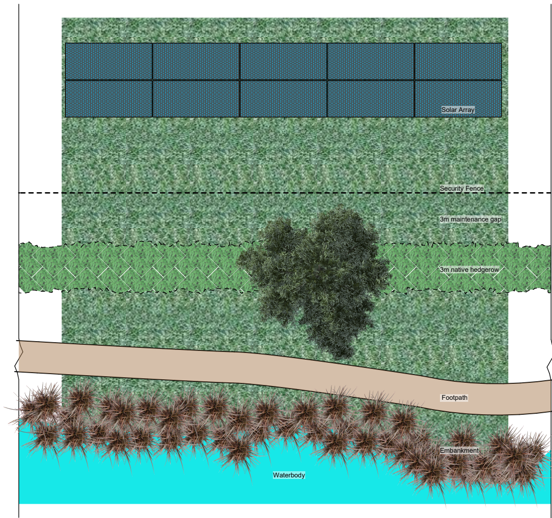
Plan View
